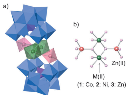
Figure 2. a) Enlarged POM unit of 1–3 , metal substituents shown as green and pink polyhedra, rest of the POM in blue/purple. and b) the central tetranuclear \{M(OH)_2(\mu_3-OH)_2\}_2\{Zn(OH_2)_2\}_2 core of POM ( M = Co ( 1 ), Ni ( 2 ), Zn ( 3 )).
